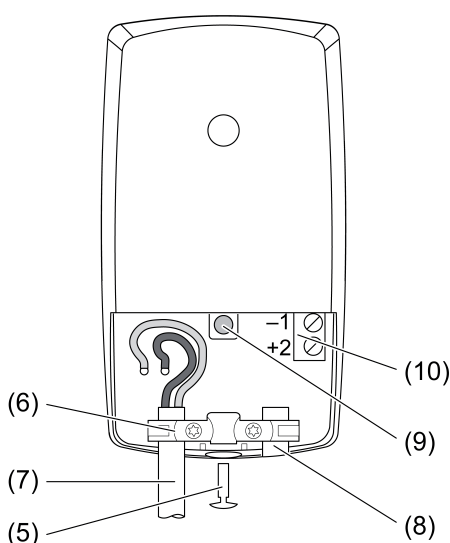
Figure 2: Valve drive with opened cover
