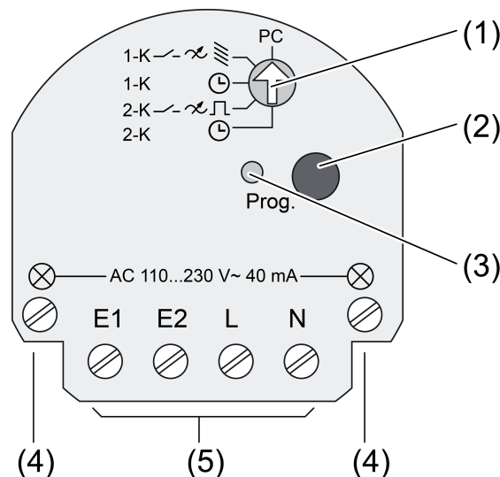
Figure 1: Front view
